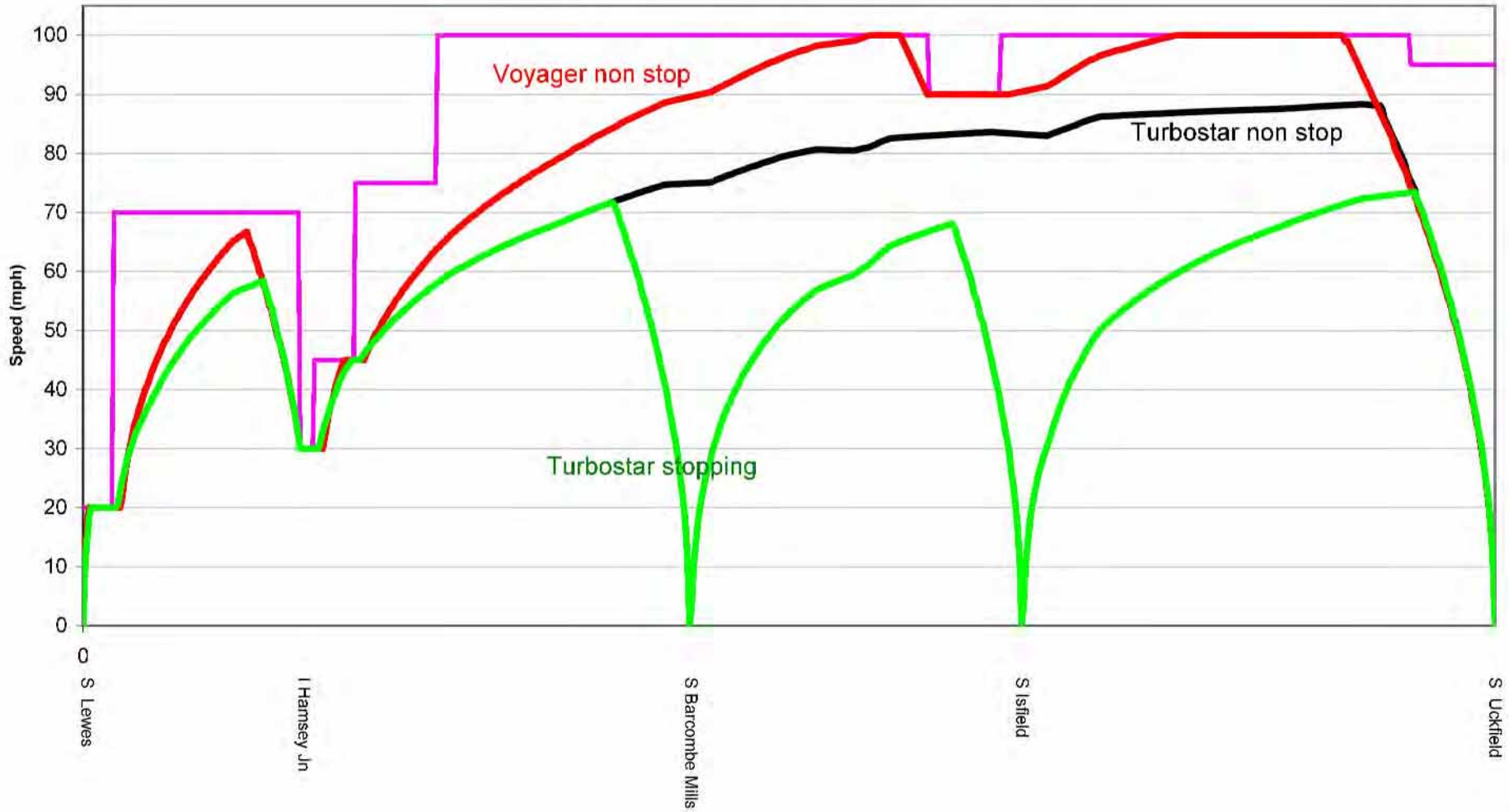
Speed Profile for Lewes to Uckfield
