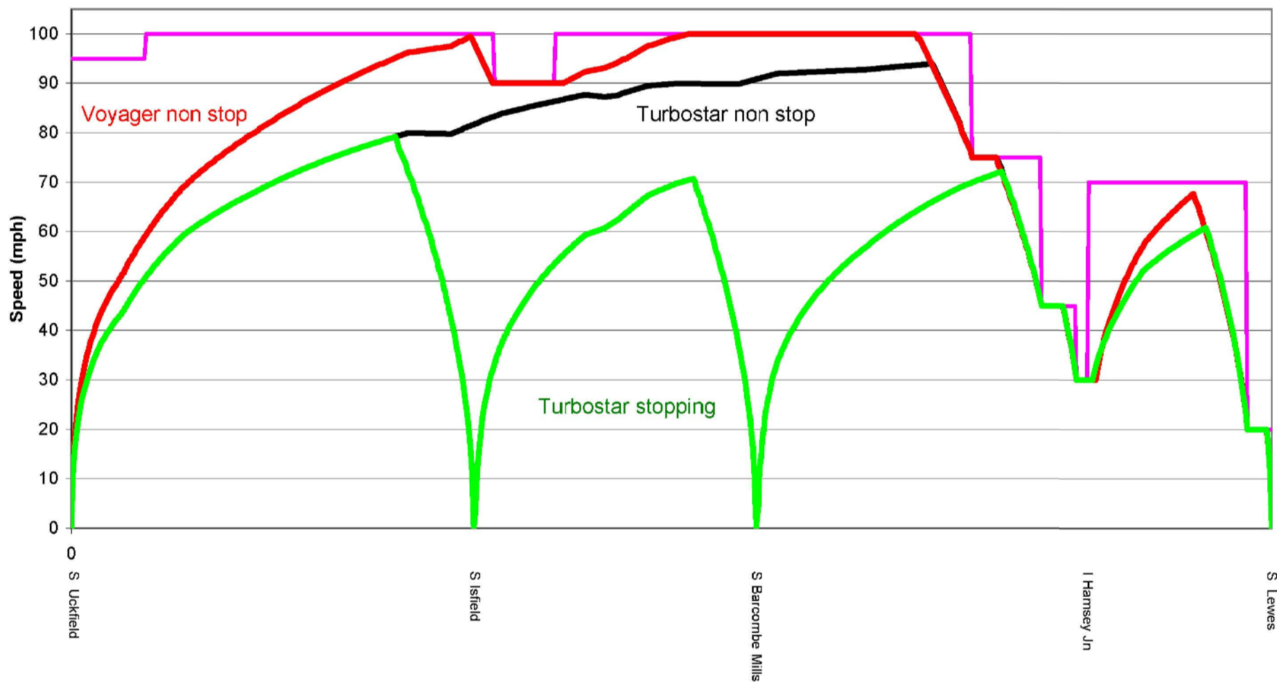
Speed Profile Uckfield - Lewes
