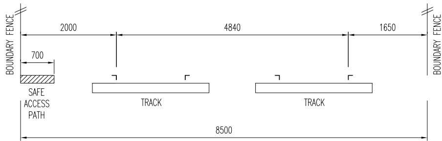
RAILWAY CORRIDOR DIAGRAM 1 (DOUBLE TRACK)
