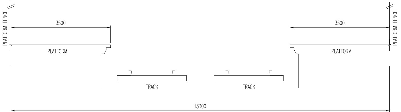
RAILWAY CORRIDOR DIAGRAM 2 (DOUBLE TRACK AT STATION)
